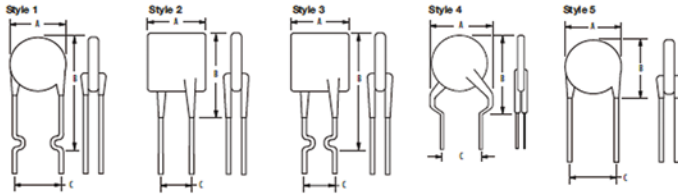
MF-RX/72 Series Radial Leaded 72 Volts 0.20 – 3.75 Amps Hold Current
