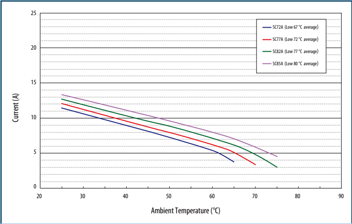
Ambient Temperature Impact on Mini-breaker Operating Currents
