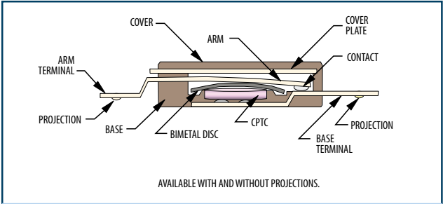
Product Structure
