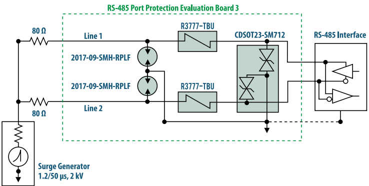
浪涌测试 2kV (1.2/50us, Rext = 80 ohms)
